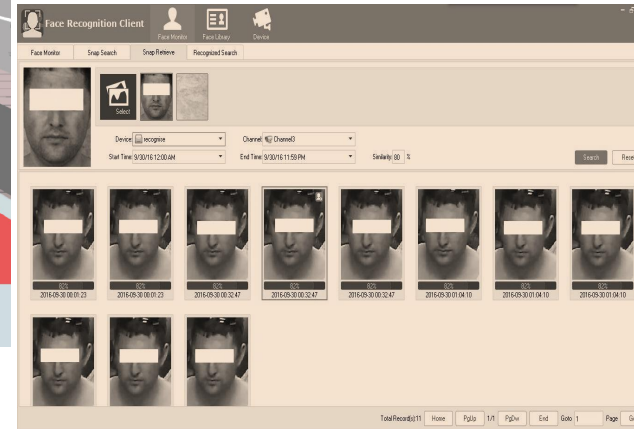
Snap Retrieve
