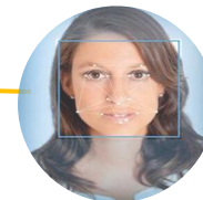
Entrance
