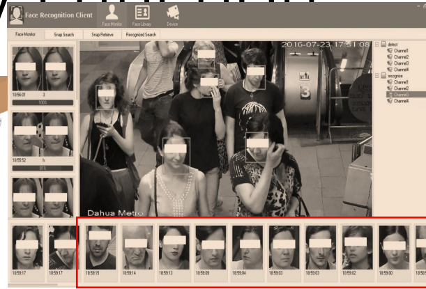
Face Capture
