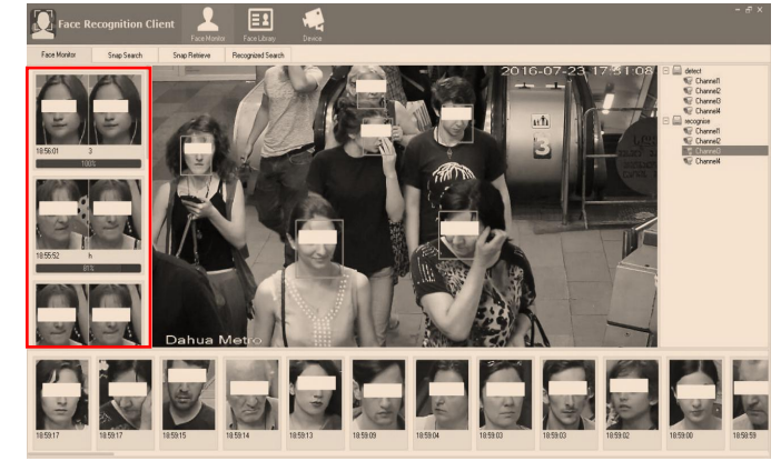
Face Comparison
