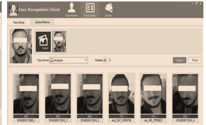
Library Search
