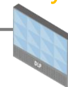
Video wall
